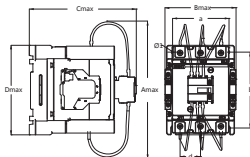
Fig.3 Overall and Installation Dimensions of NXCC-150 ~ 170 Contactor
