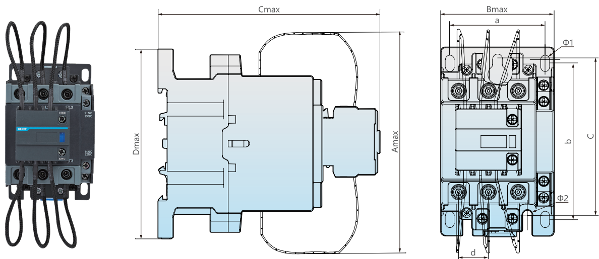
NXCC-63~115 appearance and installation dimensionsda
