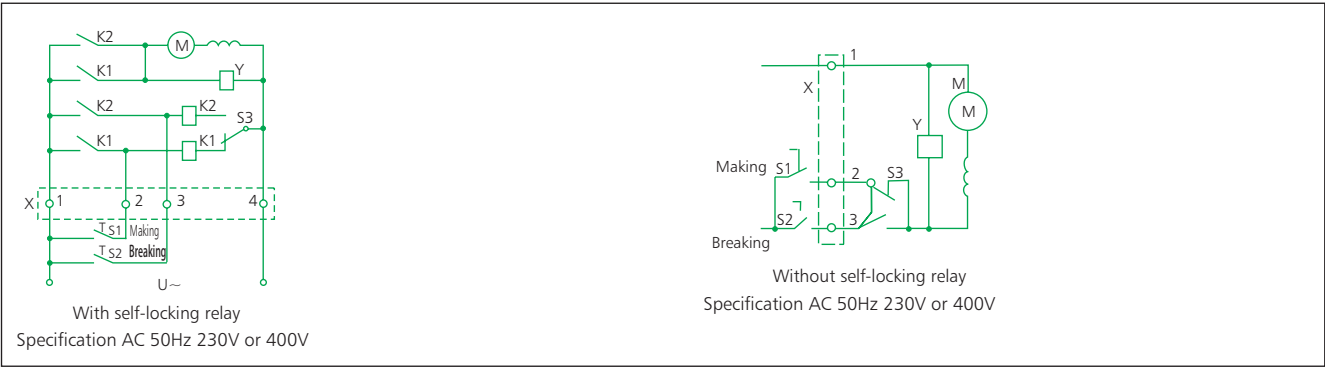
Making and breaking diagram of motor-driven operation mechanism(AC/DC)
