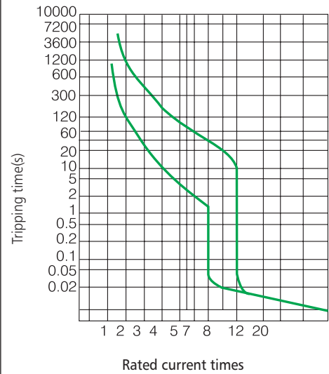
Fig.9 NM1-630, NM1-800 Characteristic Curve
