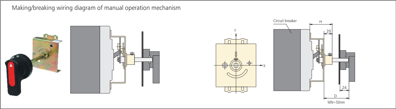
Rotary manual operation mechanism
